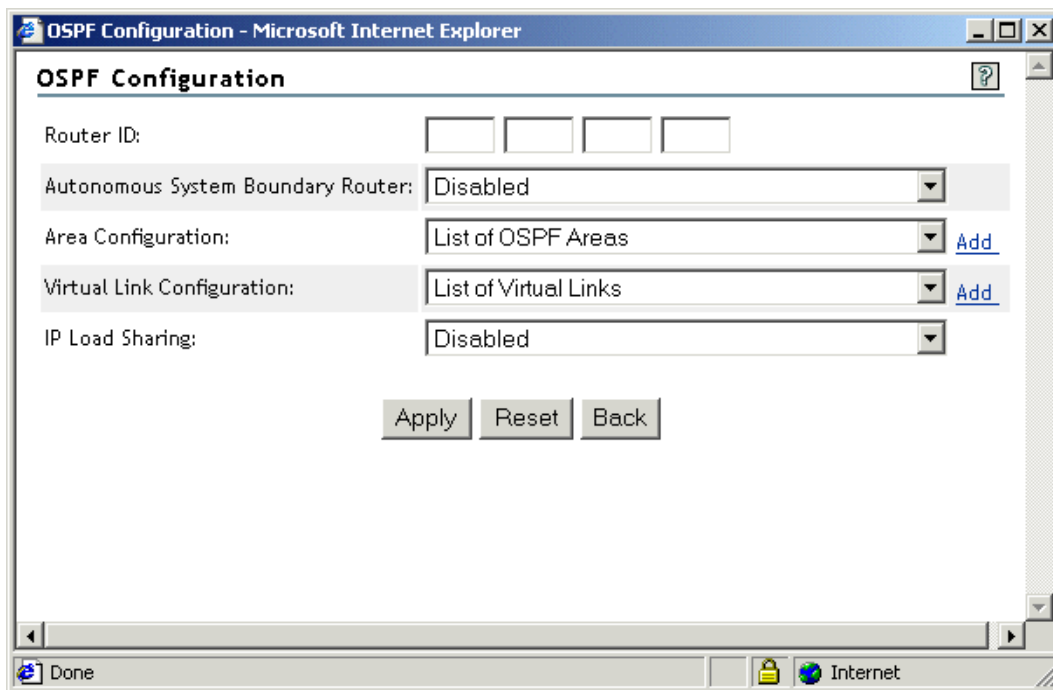
Figure 36 OSPF Configuration window
