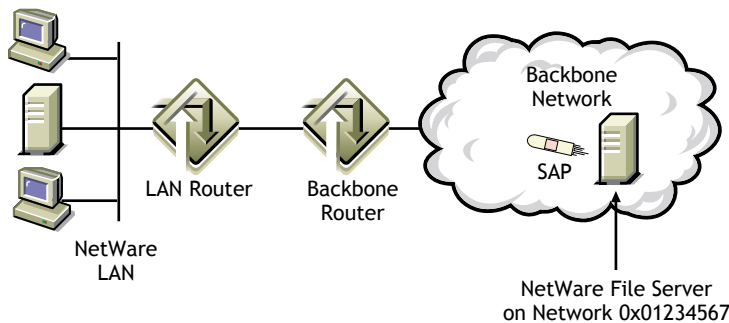
Figure 12 IPX Router Accepting and Advertising Services from a Network Not Listed in the Routing Information Table
