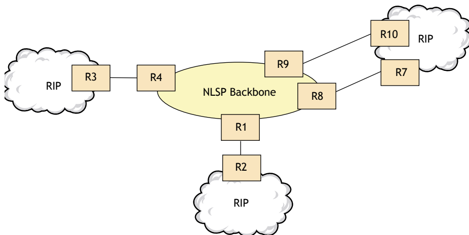
Figure 5 Aggregated Routes Topology
