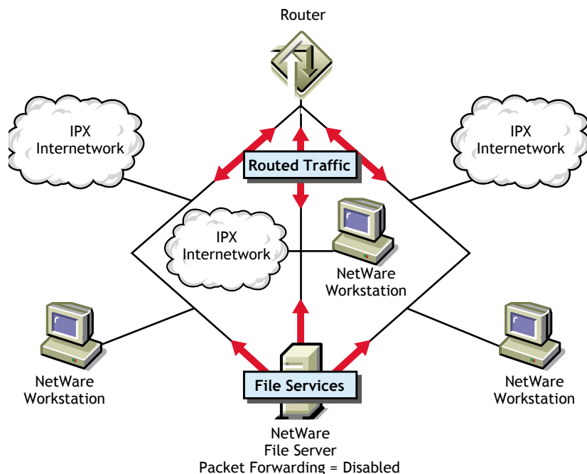
Figure 11 Turning Off IPX Packet Forwarding on a NetWare File Server
