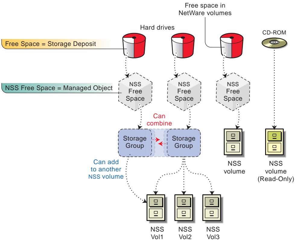
Figure 1-2 Creating Multiple NSS Volumes
