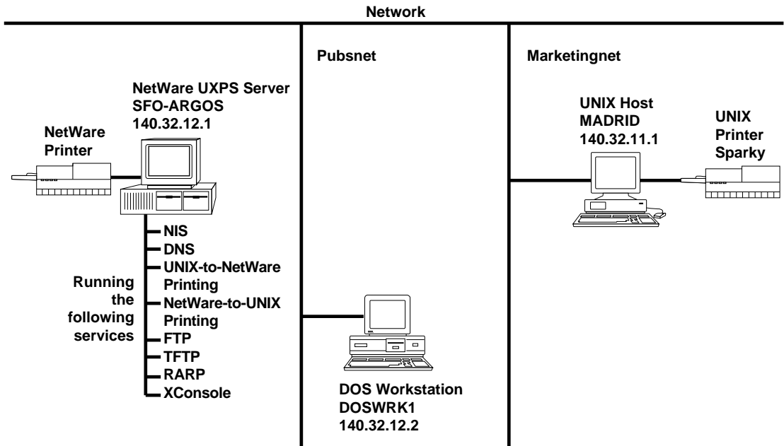
Figure 2-1 Sample Configuration
