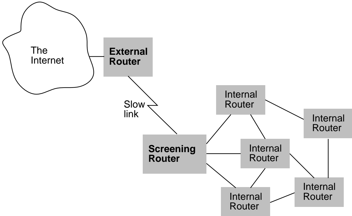
Figure 3: Organization connected to Internet via slow link
