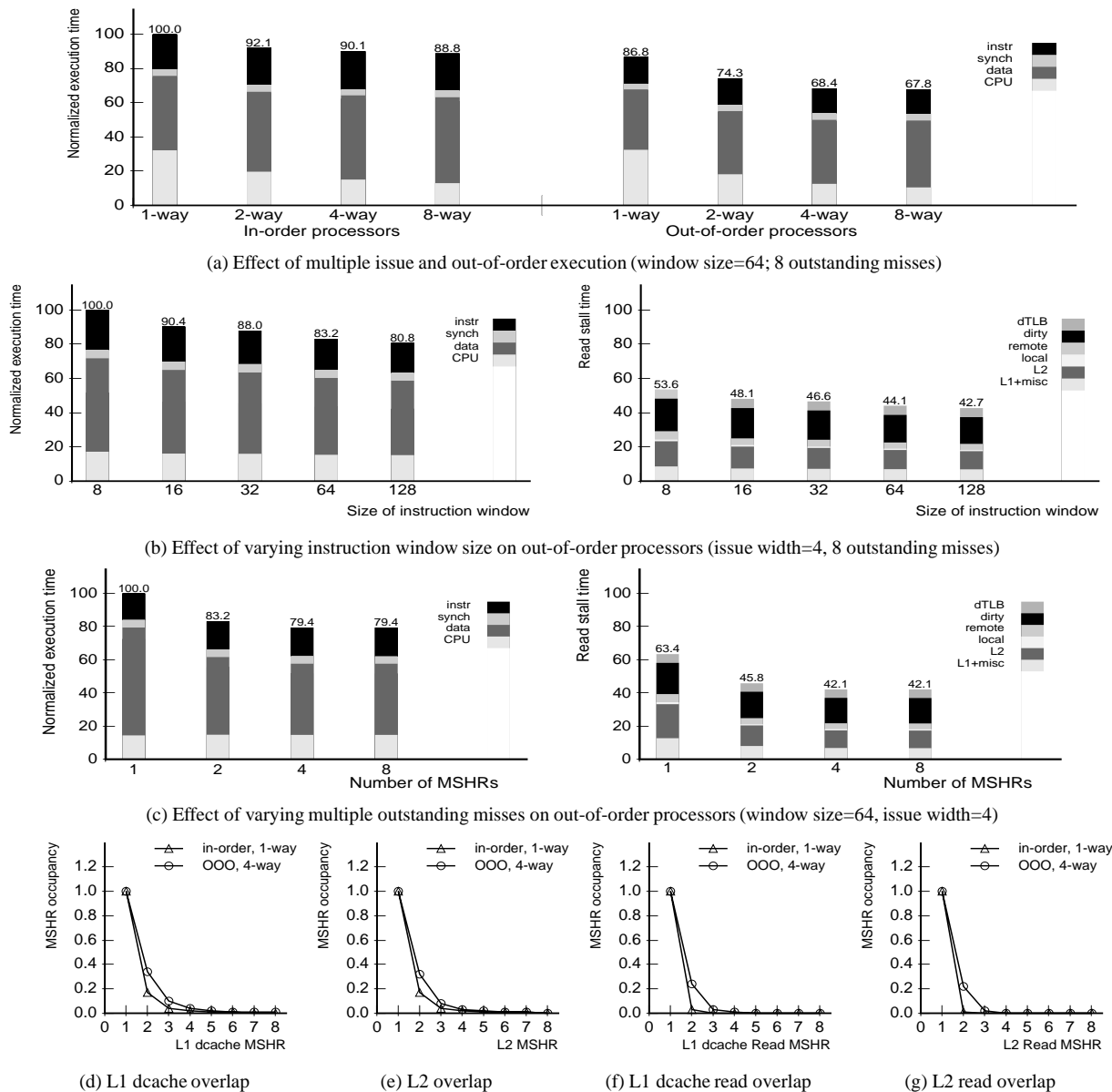
Figure 2: Impact of ILP features on OLTP performance.
