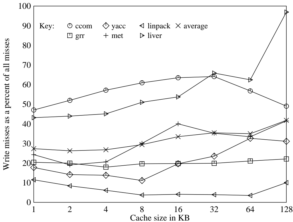
Figure 10: Write misses as a percent of all misses vs. cache size for 16B lines
