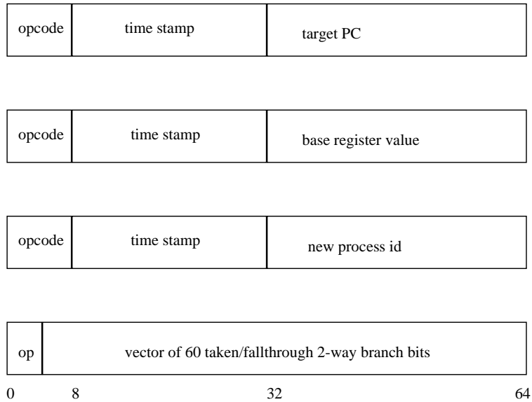
Figure 1: Formats of PatchWrx log entries. Each entry is 64 bits.
