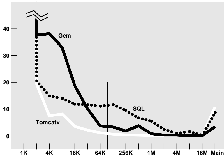
Figure 12: Incremental I-cache Hit Curves.
