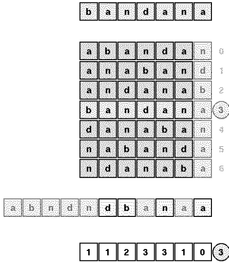
Wheeler Block Sort: Compress.obl
