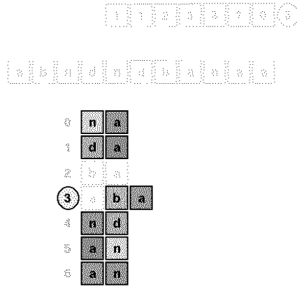
Wheeler Block Sort: WhyDecompressWorks.obl
