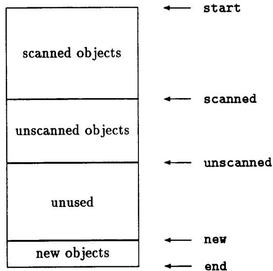
Figure 1: To-space
