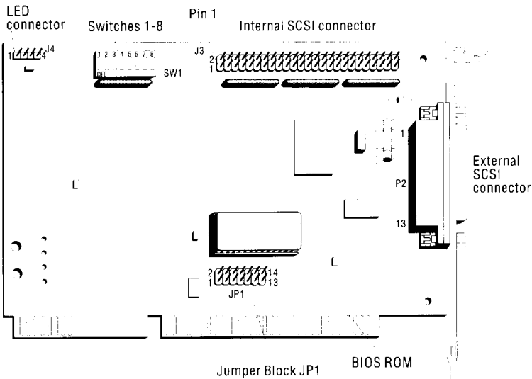
Figure 1 T160 Switch & Jumper Locations
