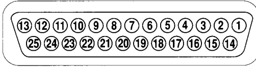
Figure 2 T160 External Connector Pinouts
