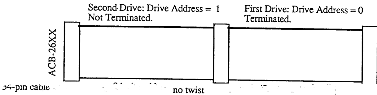
FIGURE 2-1 TWISTED VS. FLAT CABLES
