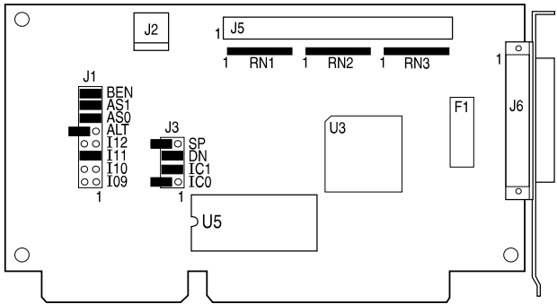
AVA-1515 Host Adapter
