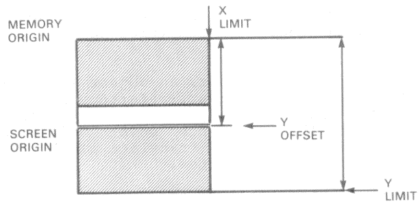
Figure 4-7 Screen-to-Memory Mapping
