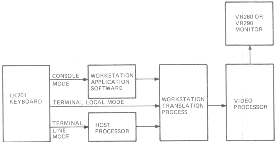
Figure B-22 Keyboard Output Processing
