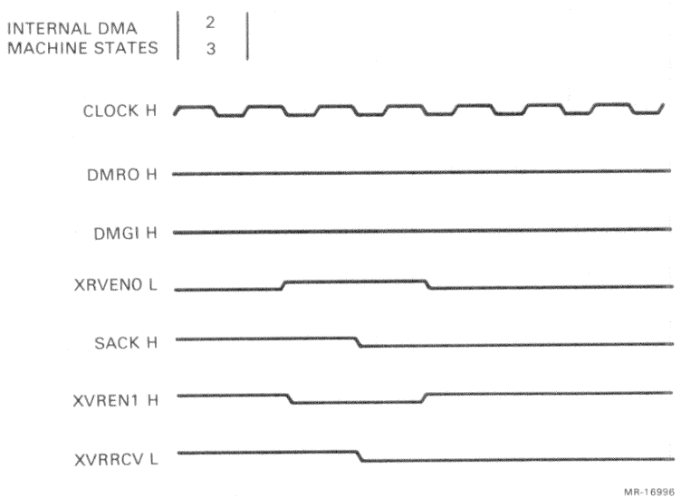
Figure 3-68 Q22-Bus Timing, Master-to-Slave Transition
