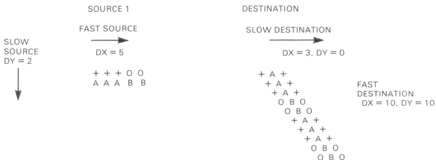
Figure 4-25 Linear Pattern
