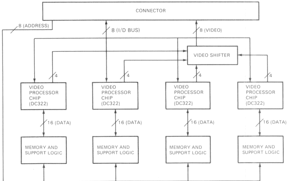
Figure 1-4 VCB02 4-Plane Module, Block Diagram
