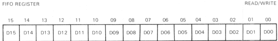
Figure 3-54 FIFO Register Bitmap
