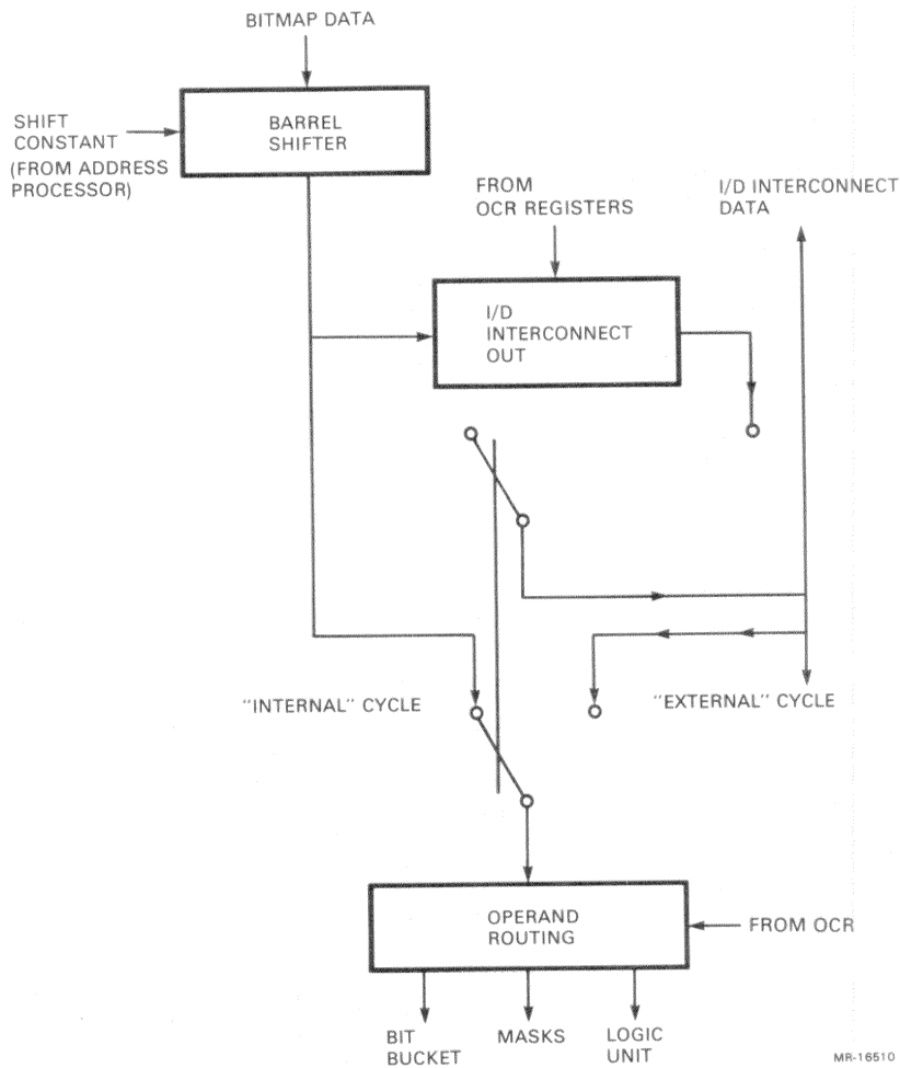
Figure 4-17 Operand Routing Functions
