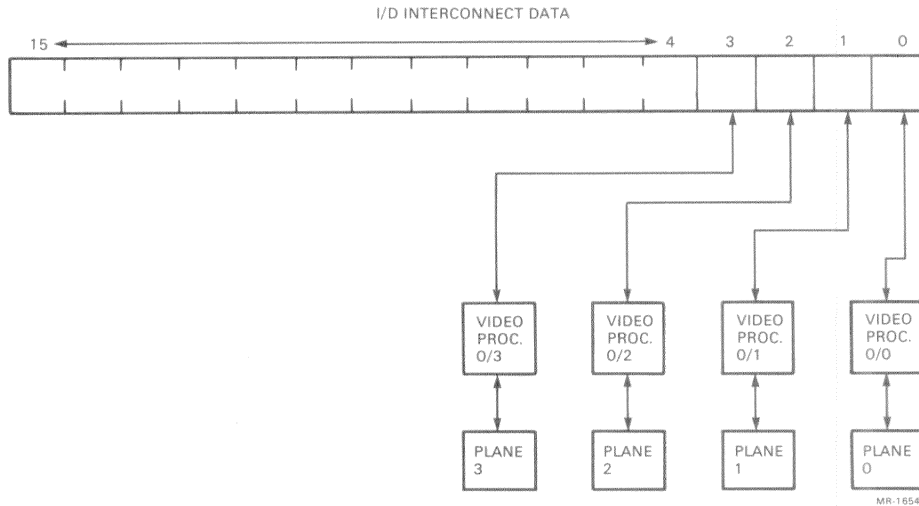
Figure 4-40 Z-Axis Addressing
