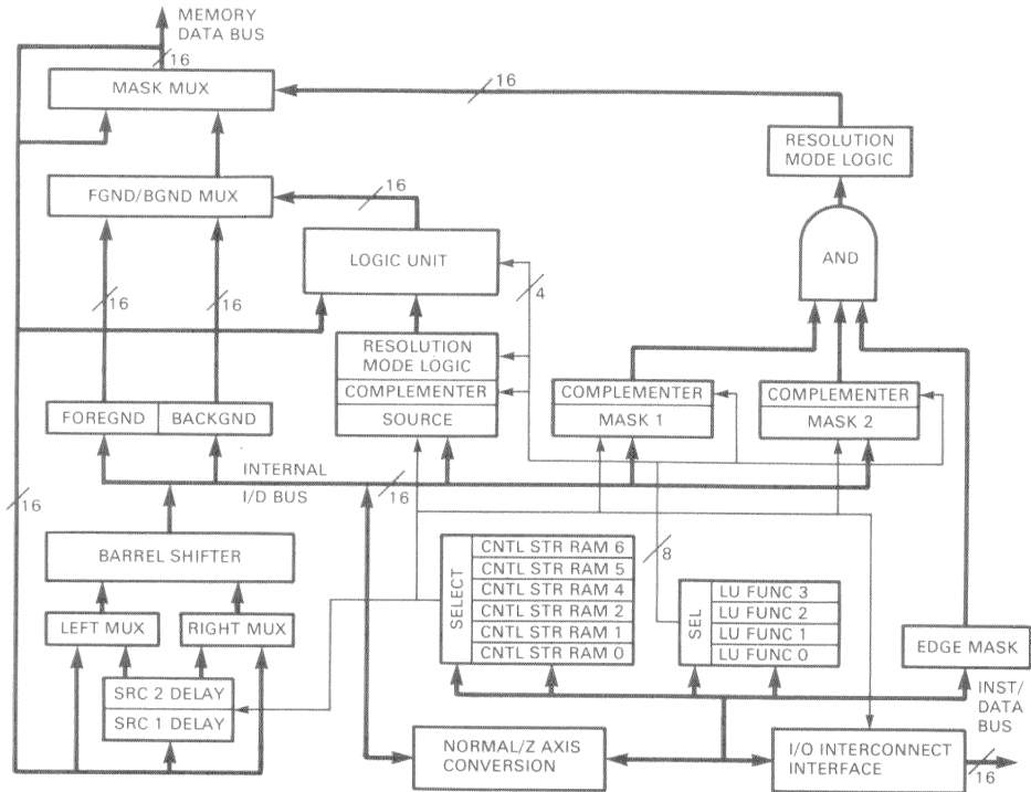
Figure 3-21 Video Processor Rasterop, Block Diagram
