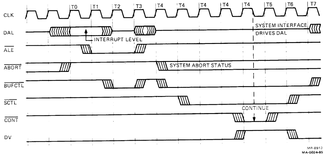
Figure 6-11 Interrupt Acknowledge Transaction
