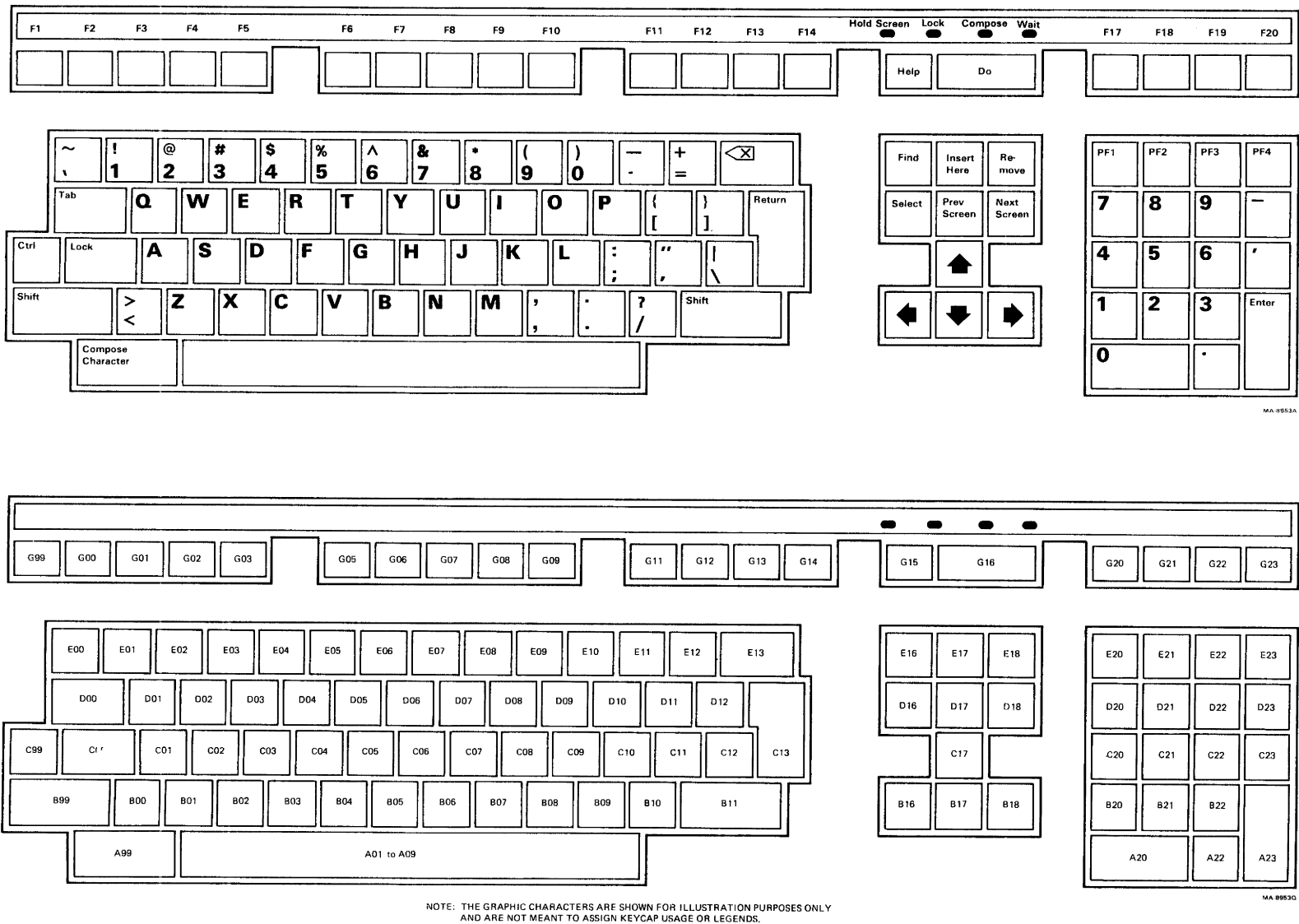
Figure 9-7 LK201-AA Keyboard Layout
