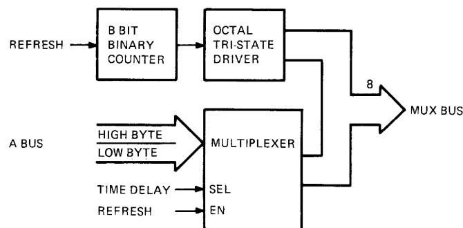
Figure 5-28 RAM Address Multiplexer 5-50
