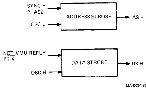
Figure 5-11 Address and Data Strobe
