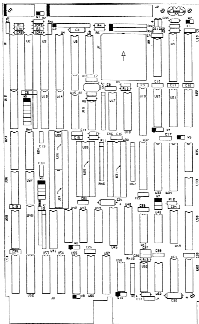
Figure 2 Jumper block location diagram hardware Rev. A
