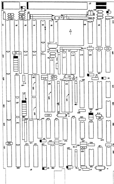
Figure 1 Jumper block location diagram hardware Rev. B
