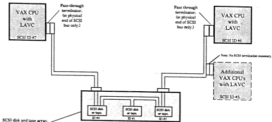
FIGURE 3 Multi-Hosting Connection Example Diagram
