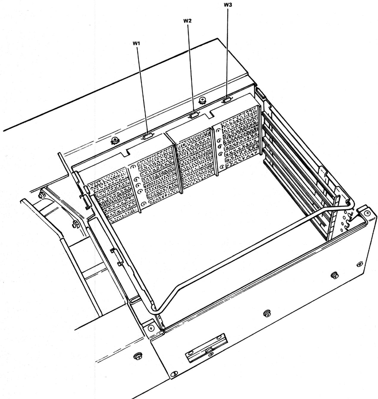
Figure 2-2 Backplane Jumpers
