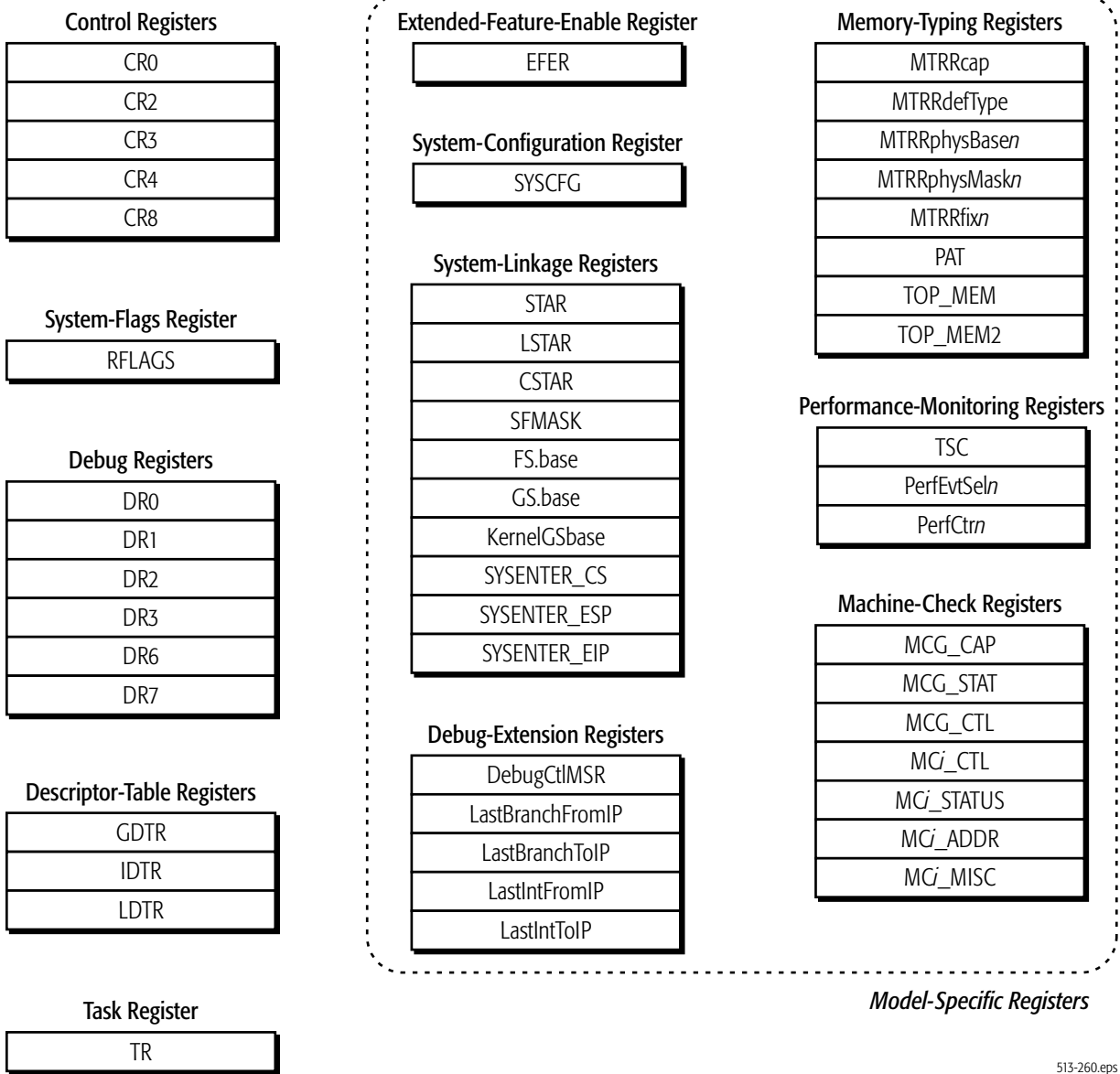
Figure 2-6. System Registers
