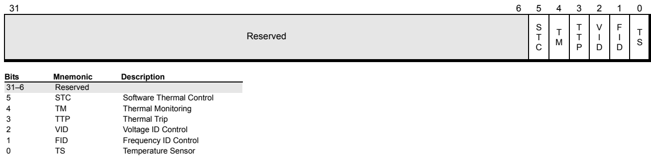
Figure 3-3. Advanced Power Management Features (EDX Register)
