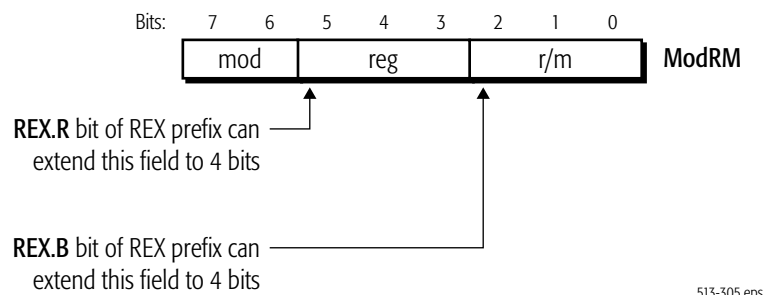
Figure 1-4. ModRM-Byte Format
