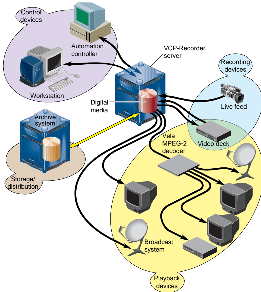
Figure 2-1 Functional Overview
