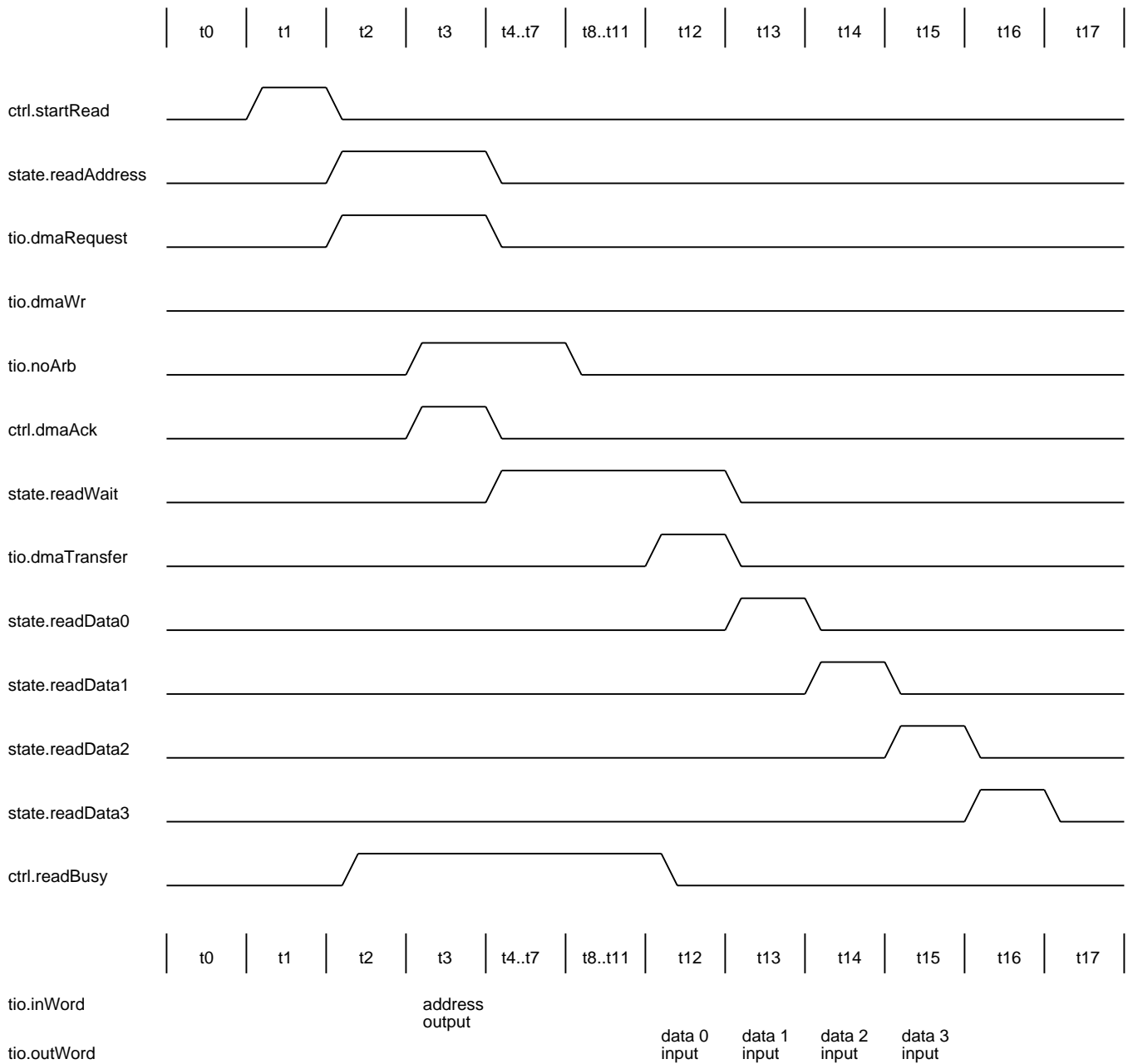
Figure 5-9: DMA Read Transaction
